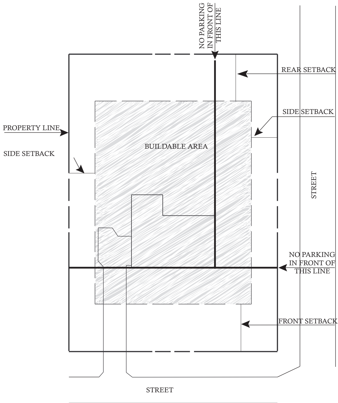
B. CORNER LOT
